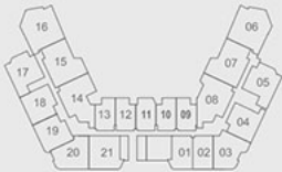
25TH-31ST TYP. FLOORS
