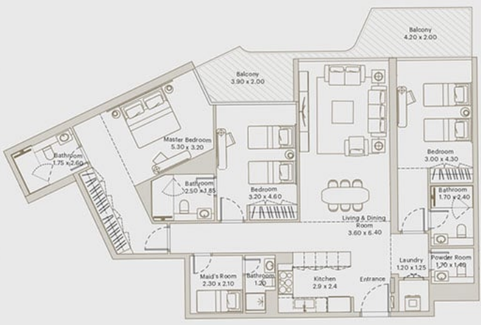
FLAT 08 @ 25TH, 27TH, 29TH & 31ST FLOOR
