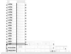
KEY SECTION
