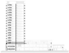
KEY SECTION
