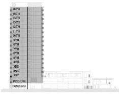
KEY SECTION
