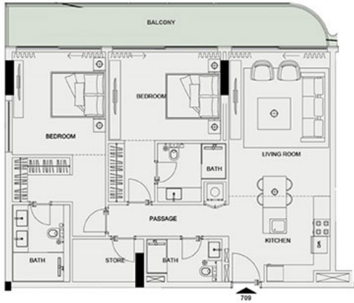
UNIT 709 - 2 BEDROOM
