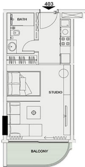
UNIT 403 - STUDIO
