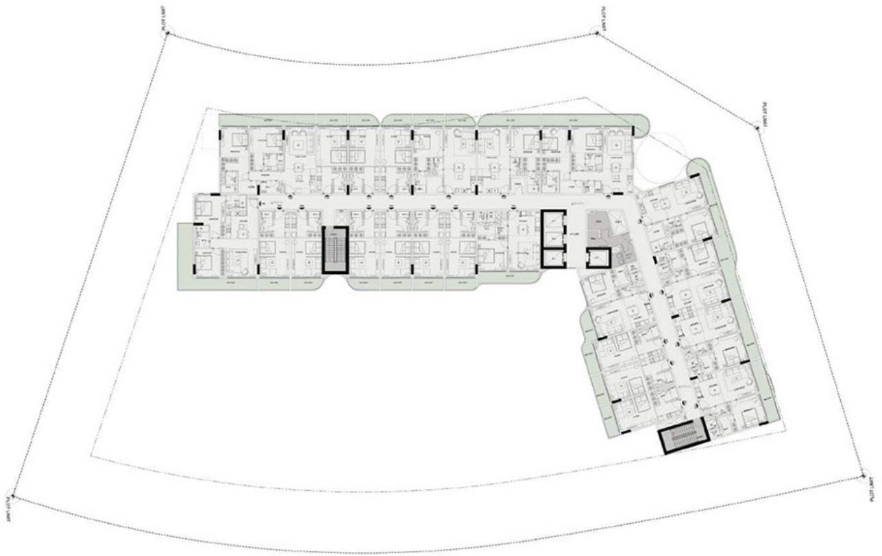
SEVENTH FLOOR PLAN
