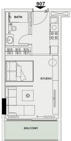
UNIT 907 - STUDIO
