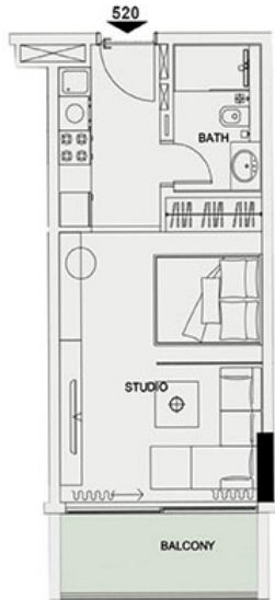
UNIT 520 - STUDIO
