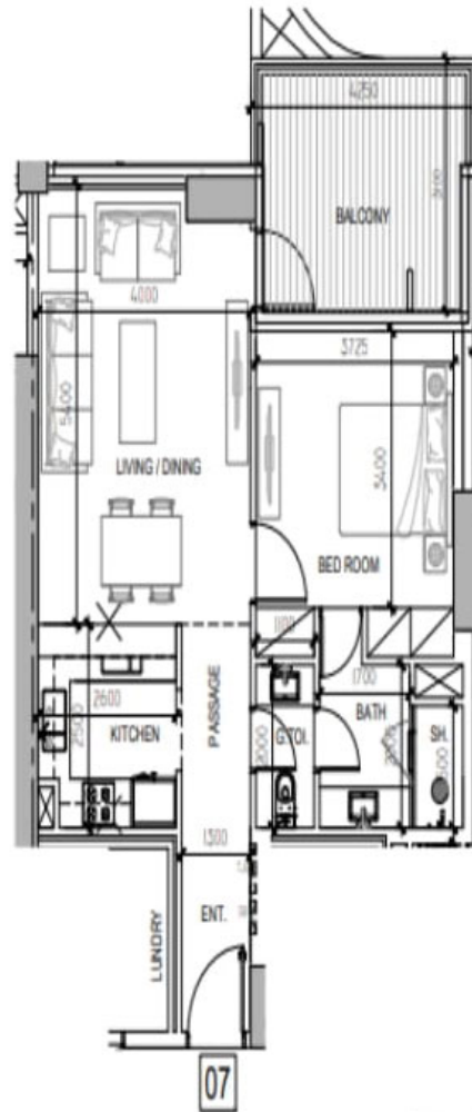
APARTMENT - 1 BED ROOM-TYPE 1B-C
