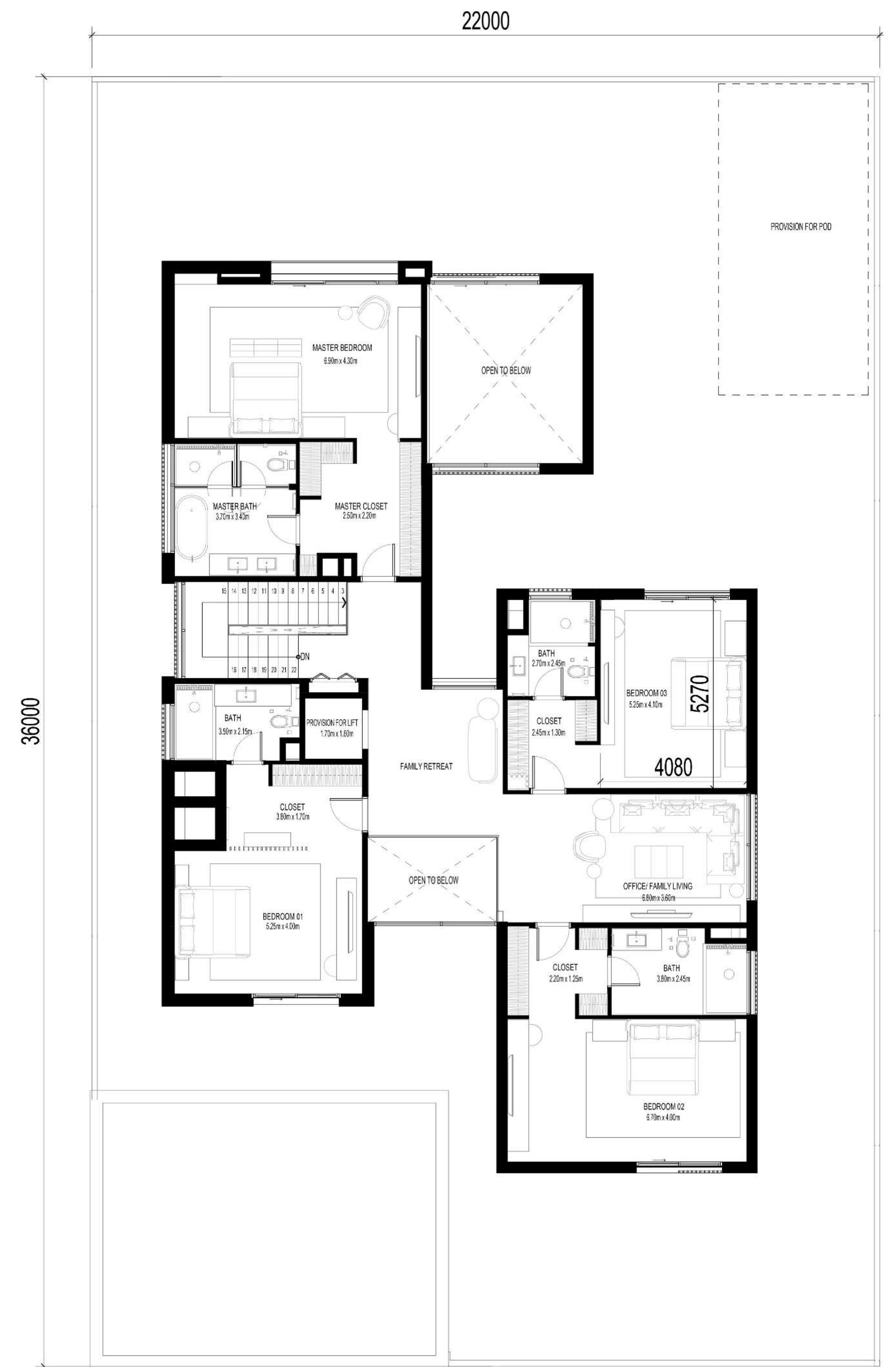
FIRST FLOOR
