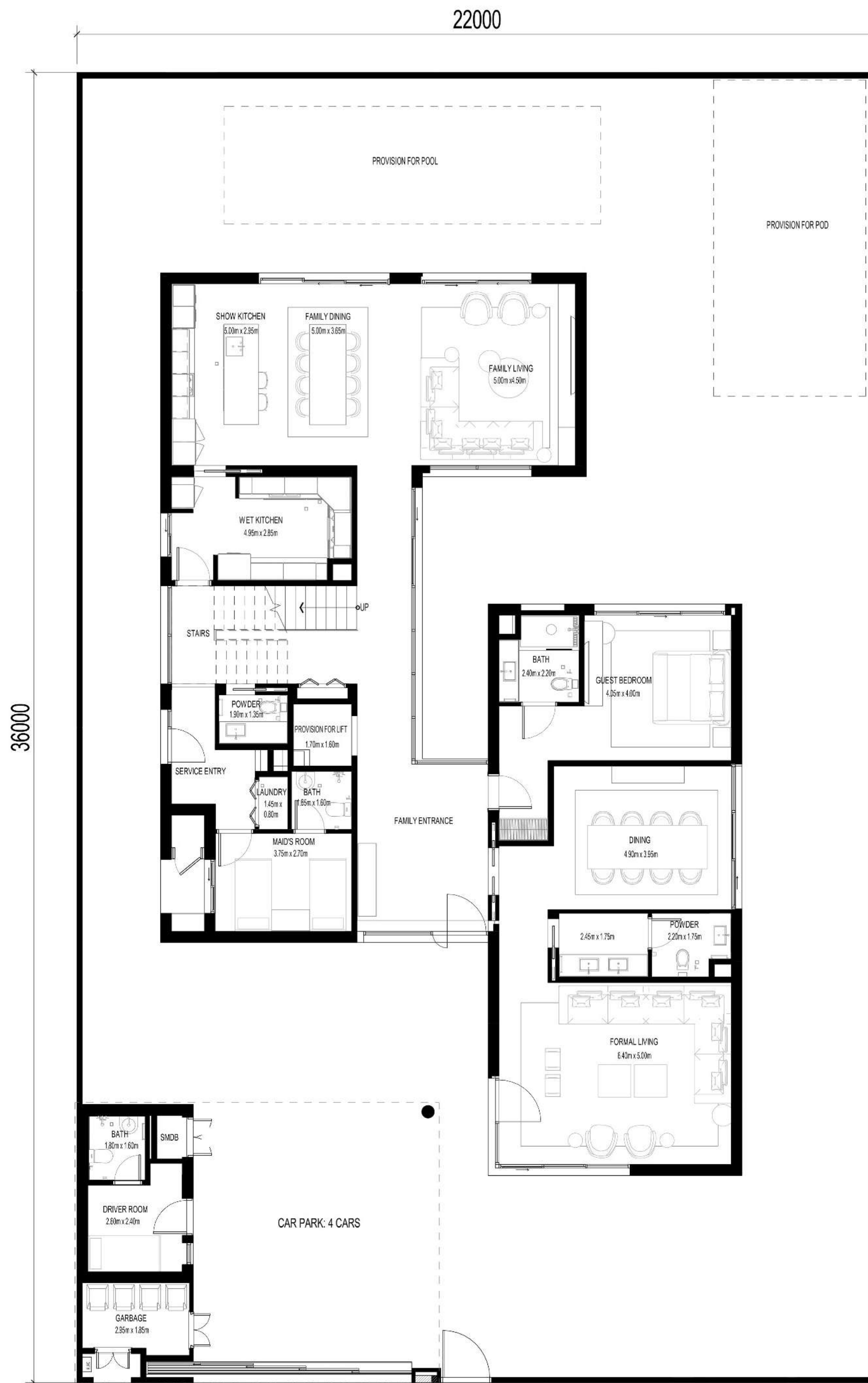
GROUND FLOOR
