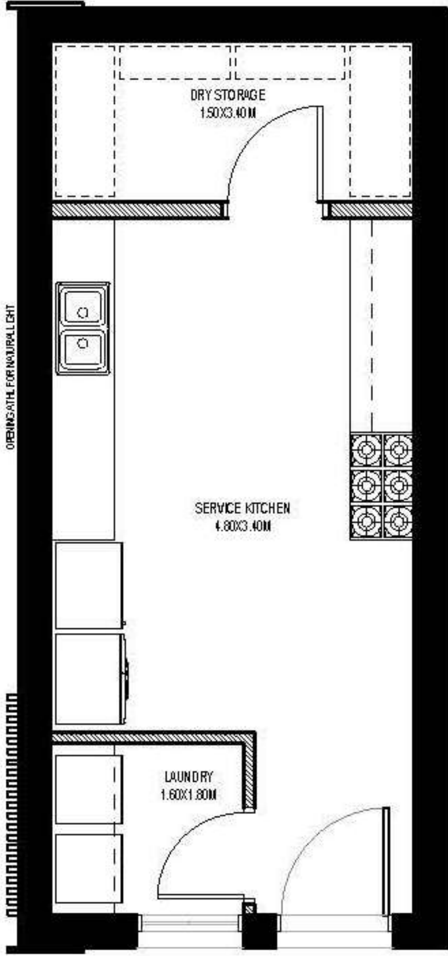
KITCHEN POD
