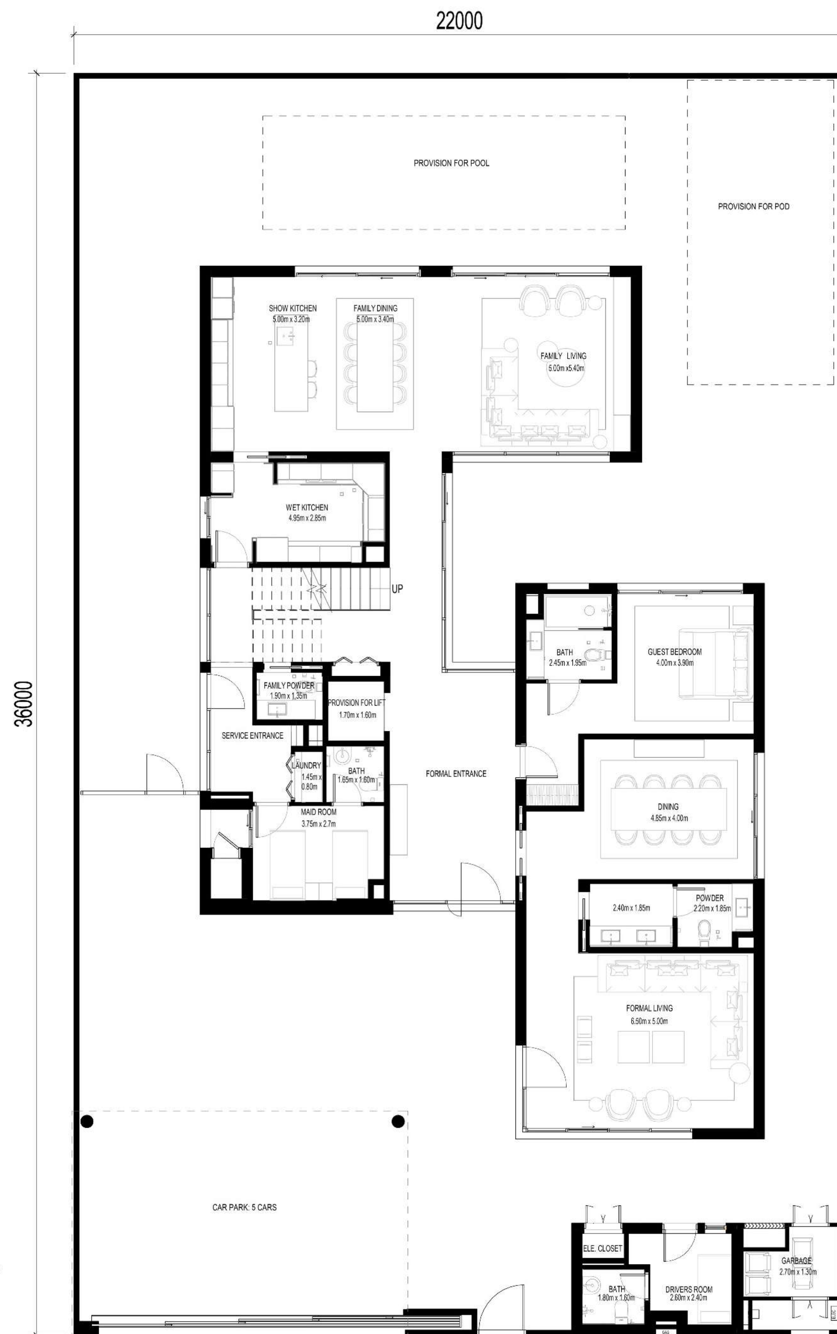
GROUND FLOOR
