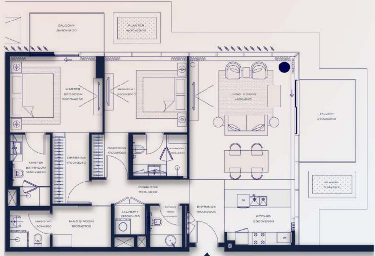
FLOOR 5
