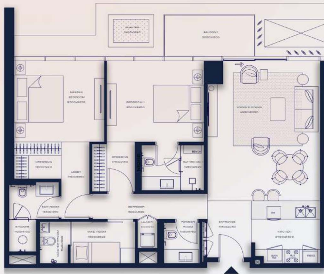
FLOOR 3
