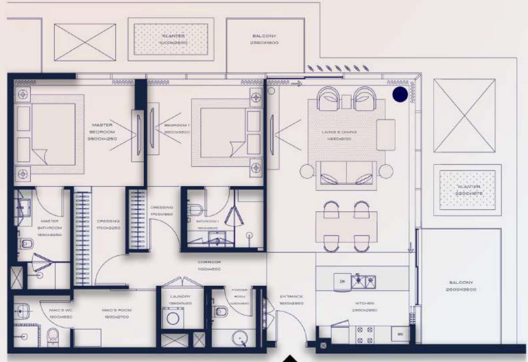
FLOOR 4
