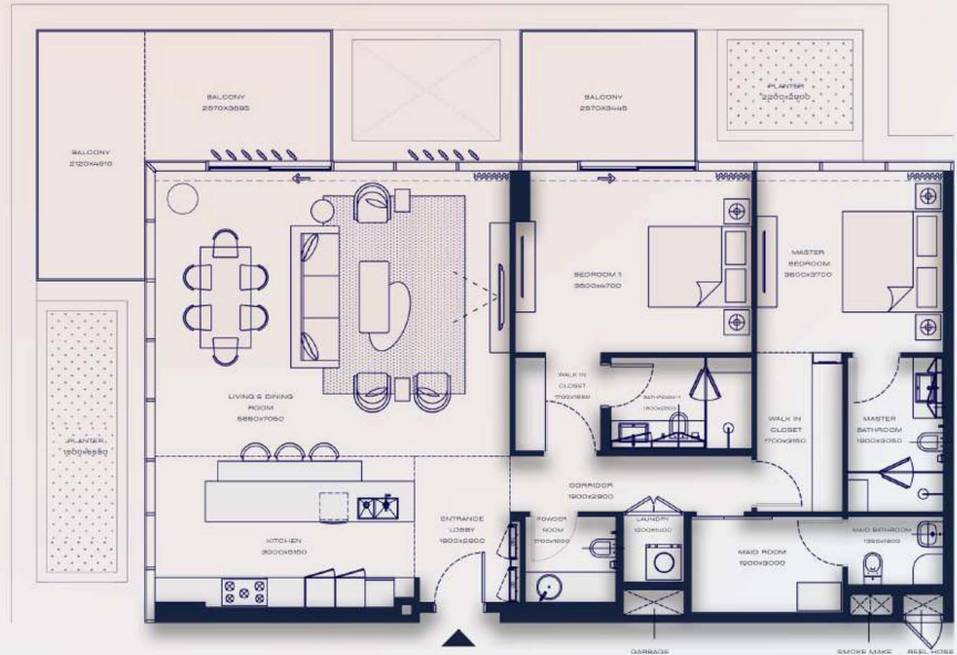
FLOOR 2
