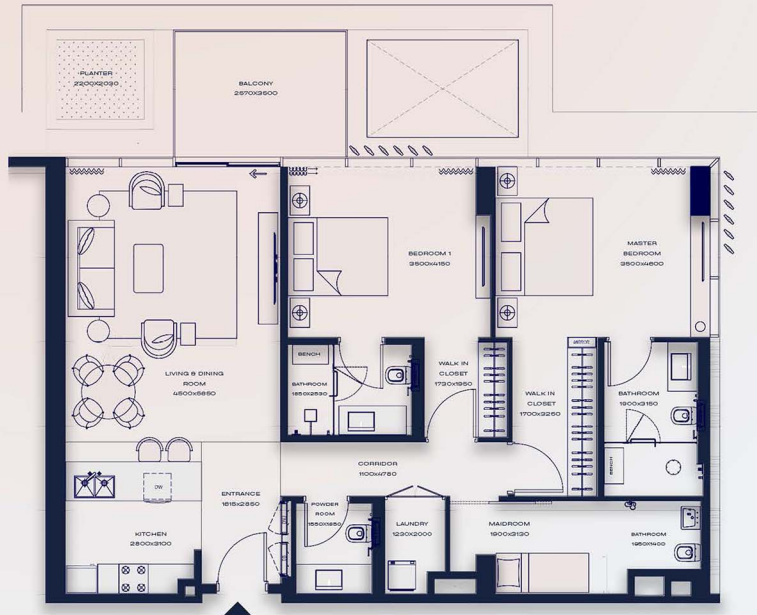
FLOOR 7
