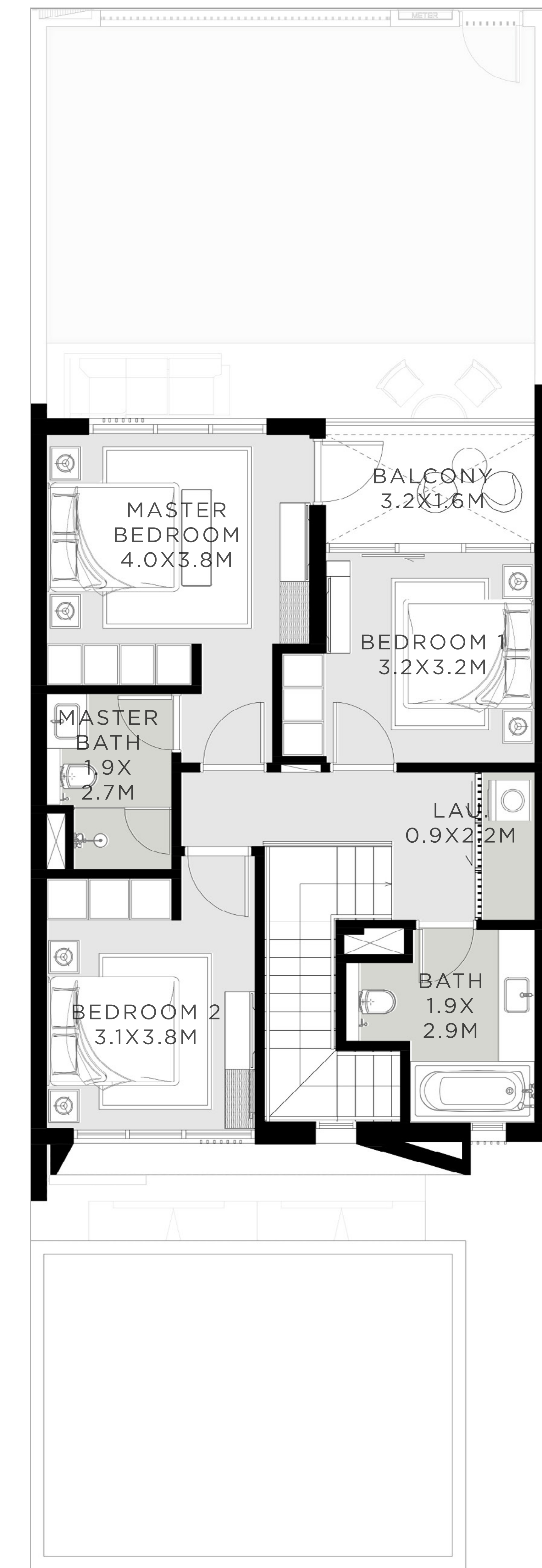
FIRST FLOOR
