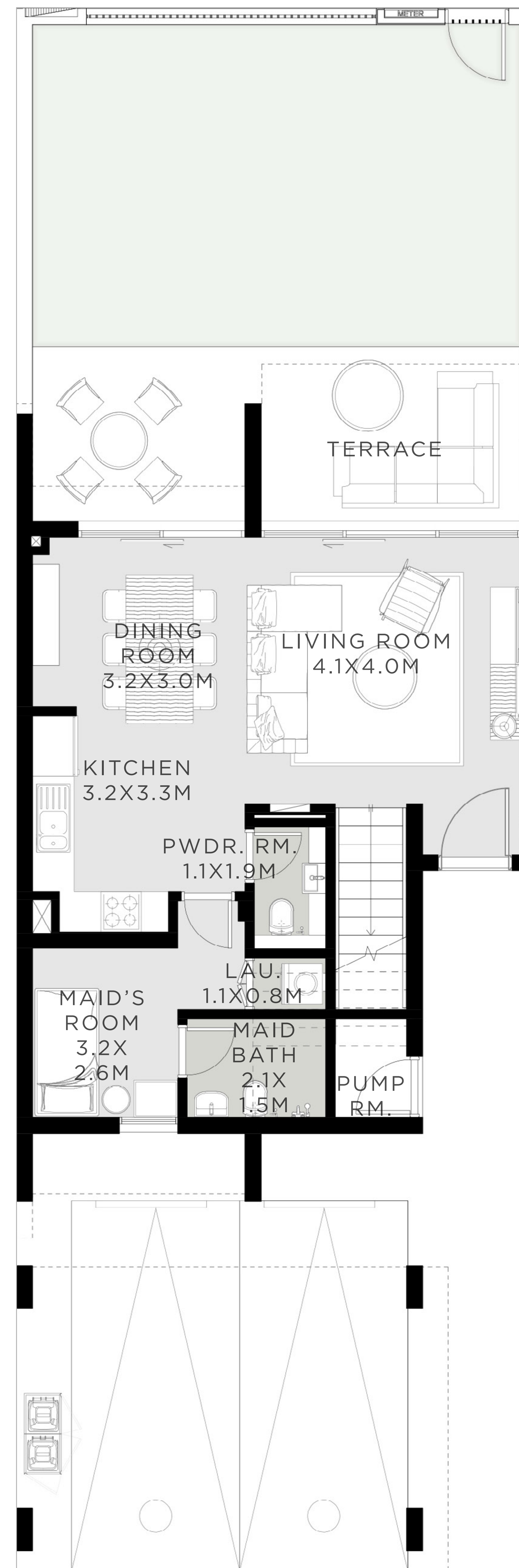
GROUND FLOOR
